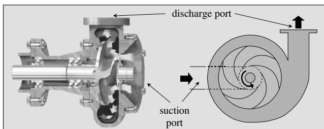
Figure 11-1 Centrifugal Pump
