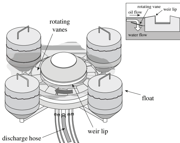
Figure 9-17 Rotating Vane Skimmer
