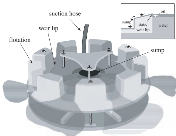
Figure 9-2 Simple Weir Skimmer
