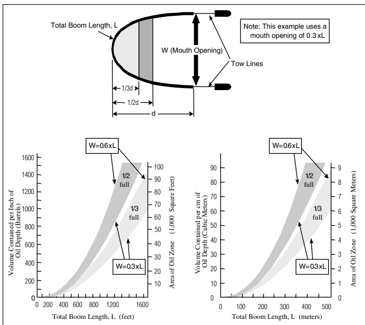
Figure 8-1 Estimating Boom Holding Capacity
