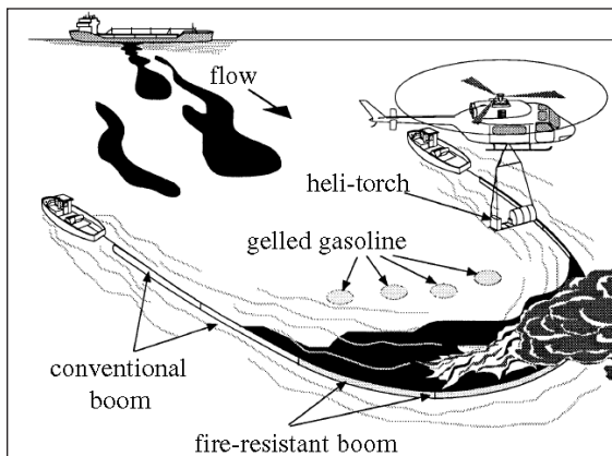
Figure 8-3 Typical In-Situ Burning Operation
