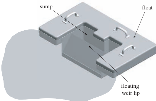
Figure 9-4 Self-Leveling Weir
