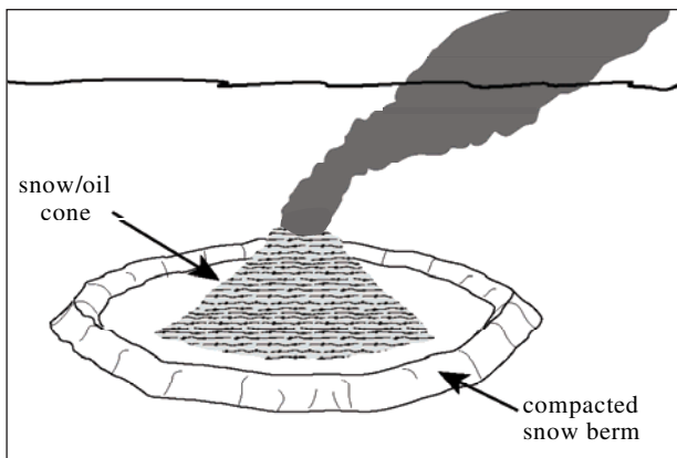
Figure 15-2 Burning Snow Cone (From EPPR 1998)
