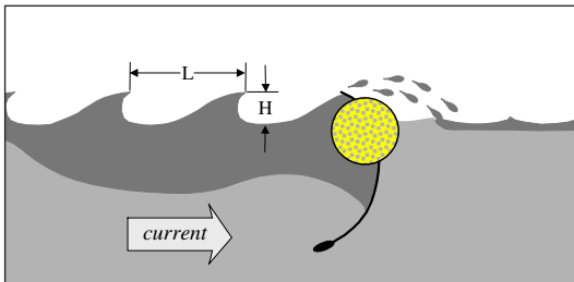
Figure 5-4 Splashover Failure
