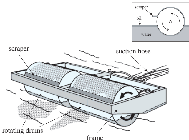
Figure 9-8 Drum Skimmer
