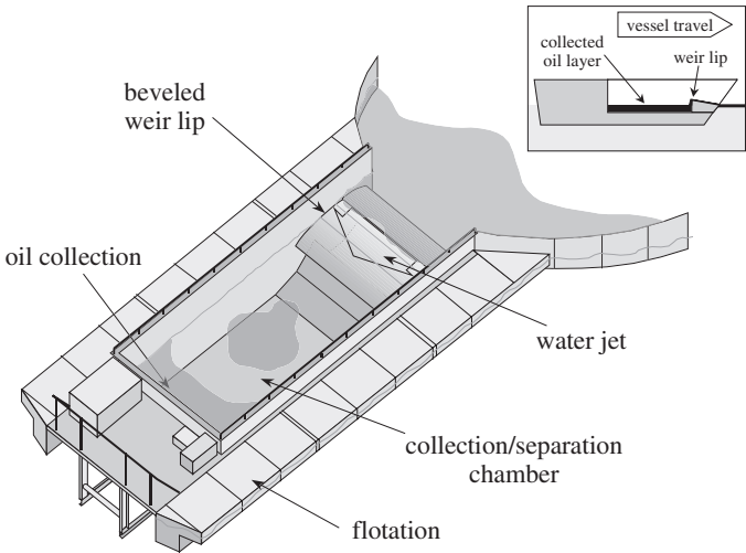
Figure 9-6 Advancing Weir Skimmer
