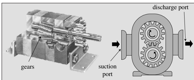
Figure 11-3 Gear Pump
