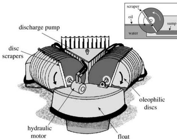
Figure 9-9 Disc Skimmer
