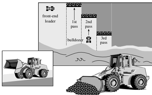
Figure 12-18 Bulldozer/Front-End Loader Combination Treatment Pattern
