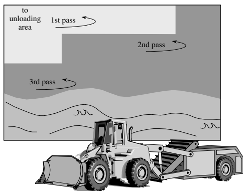
Figure 12-14 Elevating Scraper Treatment Pattern
