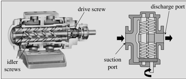
Figure 11-4 Intermeshing Screw Pump
