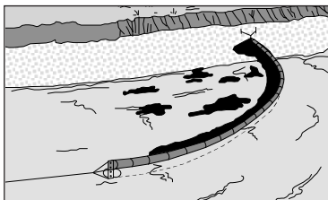
Figure 5-14 Shore-Sealing Boom
