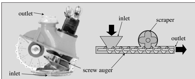
Figure 11-7 Screw/Auger Pump
