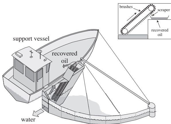
Figure 9-14 Brush Skimmer
