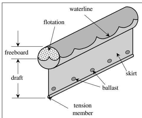
Figure 5-1 Boom Design
