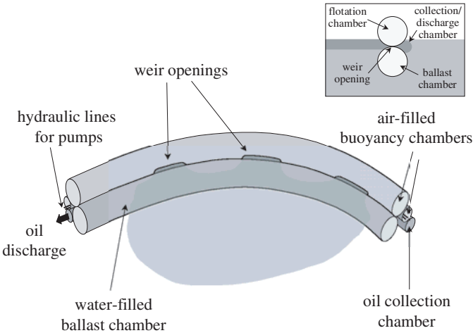
Figure 9-7 Weir Boom Skimmer
