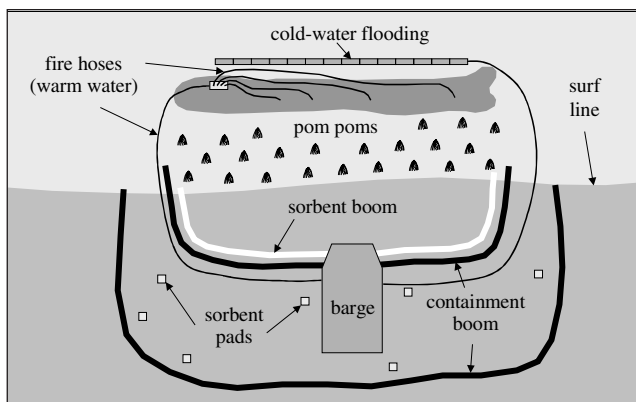
Figure 12-7 Low-Pressure, Warm-Water Washing/Cold-Water Flooding
