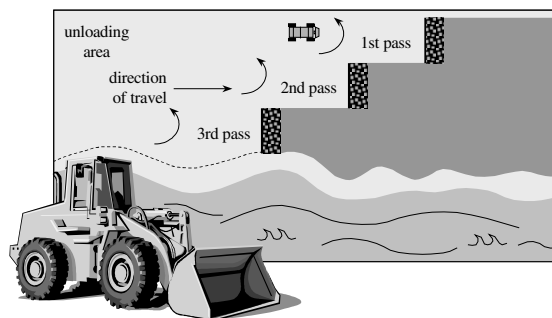
Figure 12-16 Front-End Loader Treatment Pattern
