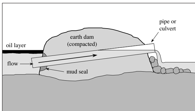
Figure 6-6 Inverted Weir
