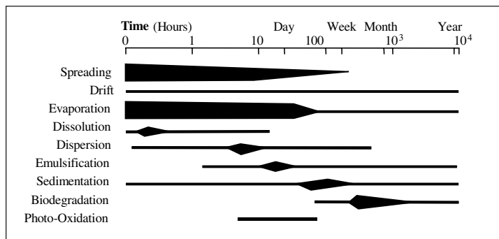
Figure 1-11 Processes Versus Time Elapsed Since the Spill
