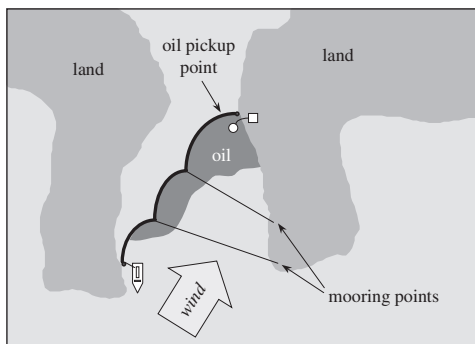
Figure 6-1 Exclusion Booming
