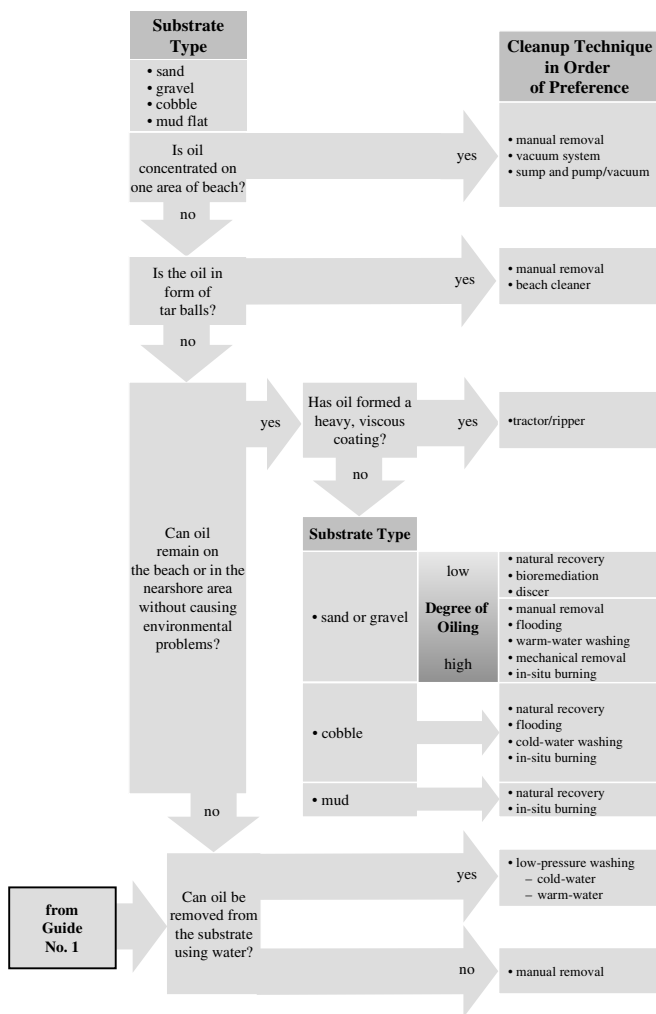
Figure 12-4 Shoreline Treatment Guide No. 2
