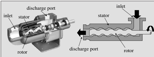
Figure 11-8 Progressive Cavity Pump
