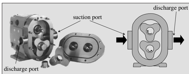
Figure 11-2 Lobe Pump
