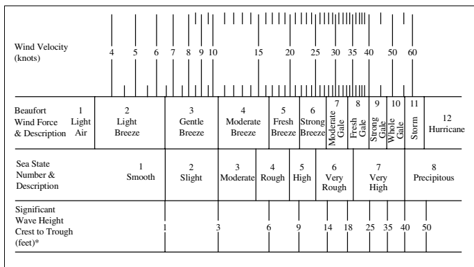
Figure 1-8 Related Wind and Wave Conditions in Fully Developed Seas
