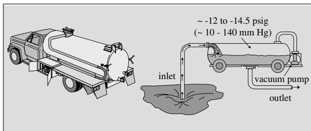
Figure 11-12 Vacuum Truck
