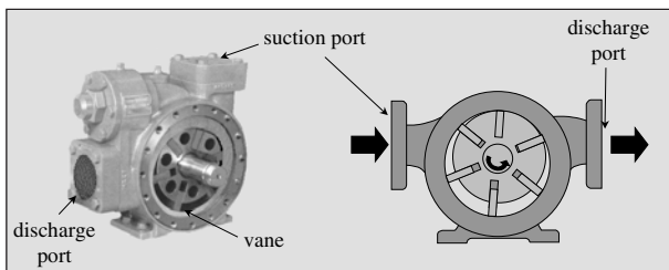
Figure 11-5 Vane Pump
