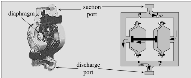
Figure 11-10 Diaphragm Pump
