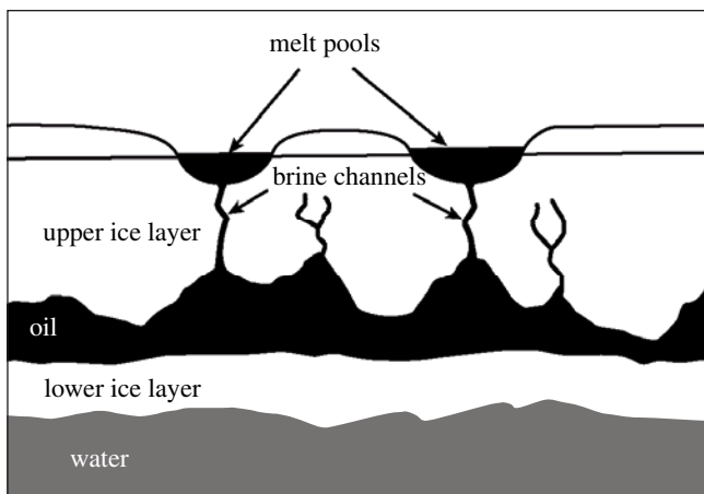
Figure 15-1 Melt Pools and Encapsulated Oil (From EPPR 1998)
