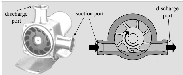
Figure 11-6 Flexible Impeller Pump
