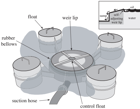
Figure 9-3 Self-Leveling Weir
