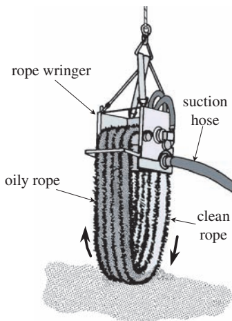
Figure 9-11 Vertical Rope Mop Skimmer
