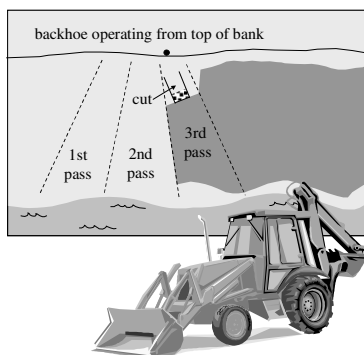
Figure 12-19 Backhoe with Front Bucket Treatment Pattern
