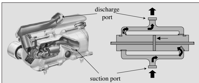
Figure 11-9 Reciprocating Pump
