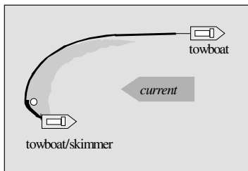
Figure 5-13 J-Booming
