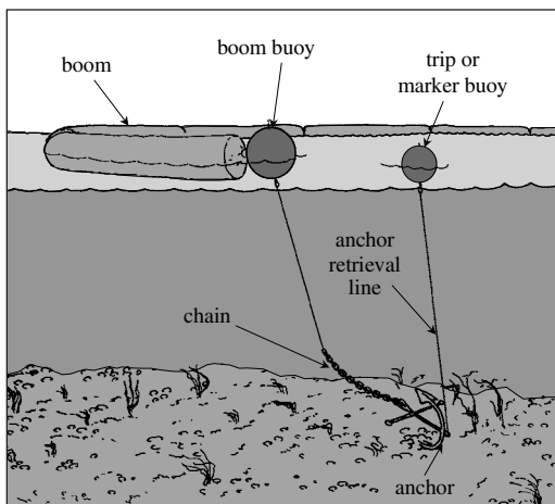
Figure 5-16 Boom Anchoring Assembly
