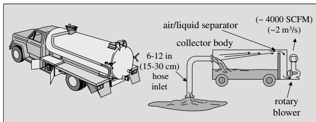
Figure 11-13 Air Conveyor
