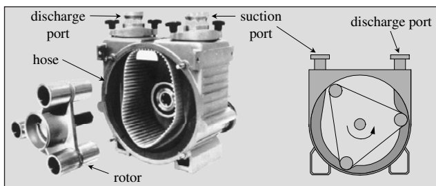
Figure 11-11 Peristaltic Pump
