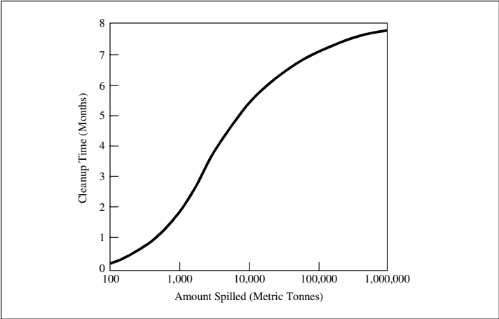
Figure 1-6 Spill Size Versus Duration of Cleanup
