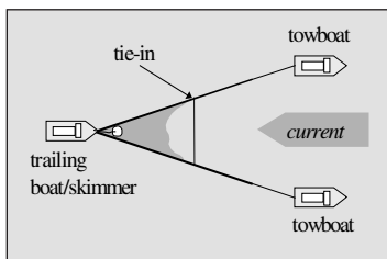
Figure 5-12 V-Booming
