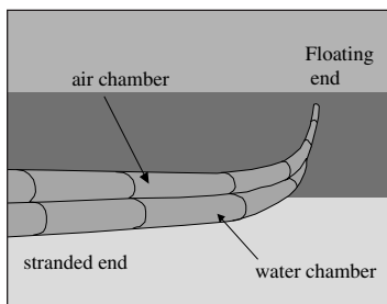
Figure 6-4 Shore-Sealing Boom
