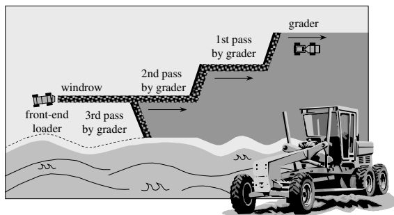
Figure 12-17 Motor Grader/Front-End Loader Combination Treatment Pattern
