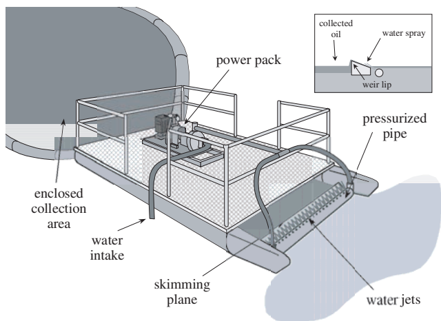
Figure 9-15 Water Jet Skimmer
