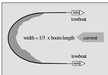
Figure 5-11 U-Booming
