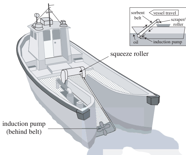
Figure 9-13 Sorbent Lifting Belt
