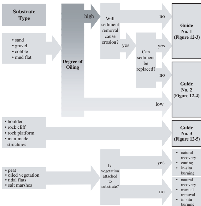
Figure 12-2 Shoreline Treatment Guide Key
