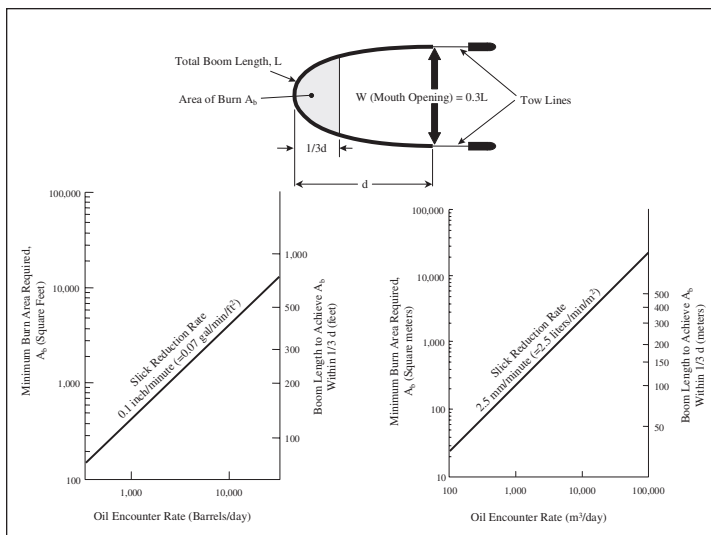
Figure 8-2 Estimating Area Required for Various Oil Encounter Rates
