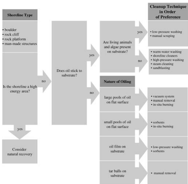
Figure 12-5 Shoreline Treatment Guide No. 3
