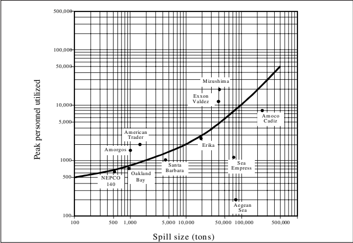
Figure 1-5 Peak Personnel Versus Amount Spilled
