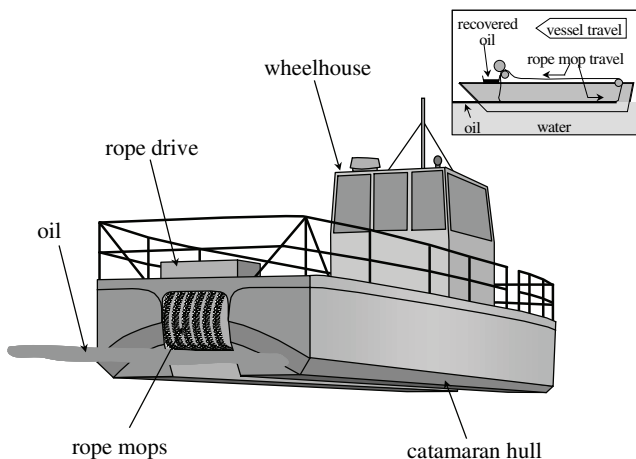
Figure 9-12 ZRV Rope Mop Skimmer
