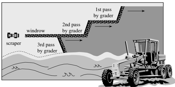
Figure 12-15 Motor Grader/Elevating Scraper Combination Treatment Pattern
