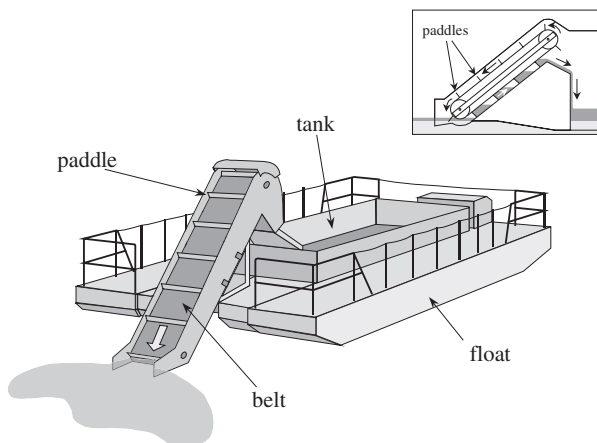
Figure 9-18 Paddle Belt Skimmer
