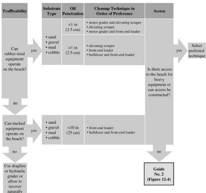
Figure 12-3 Shoreline Treatment Guide No. 1
