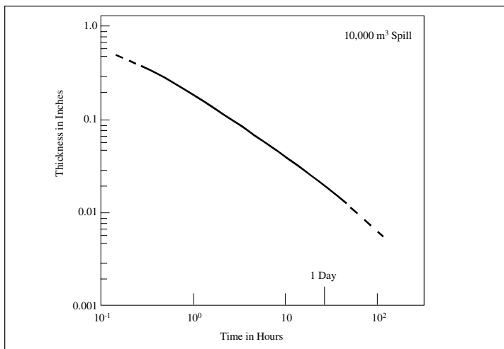
Figure 1-9 Behavior of the Thick Part of a Slick of Crude Oil on Water (From Mackay et al., Oil Spill Processes and Models, University of Toronto. Figure 1-9 is based on the first 48 hours of concentric thick and thin slicks of medium crude under calm seas and low winds.)
