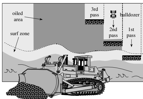
Figure 12-13 Bulldozer Treatment Pattern
