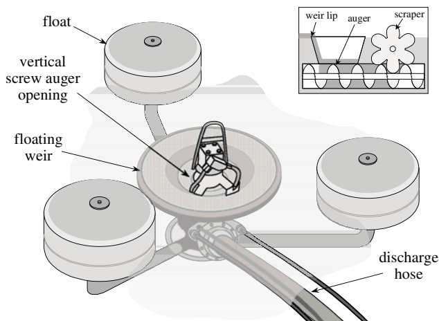
Figure 9-5 Weir with Integral Screw Auger
