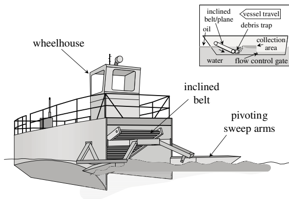
Figure 9-16 Submersion Plane/Belt Skimmer
