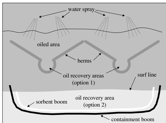
Figure 12-6 Low Pressure Flushing
