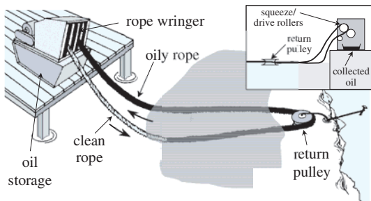
Figure 9-10 Rope Mop Skimmer
